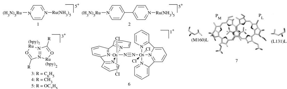
Figure 3. MVCs that have been probed by Stark spectroscopy.
