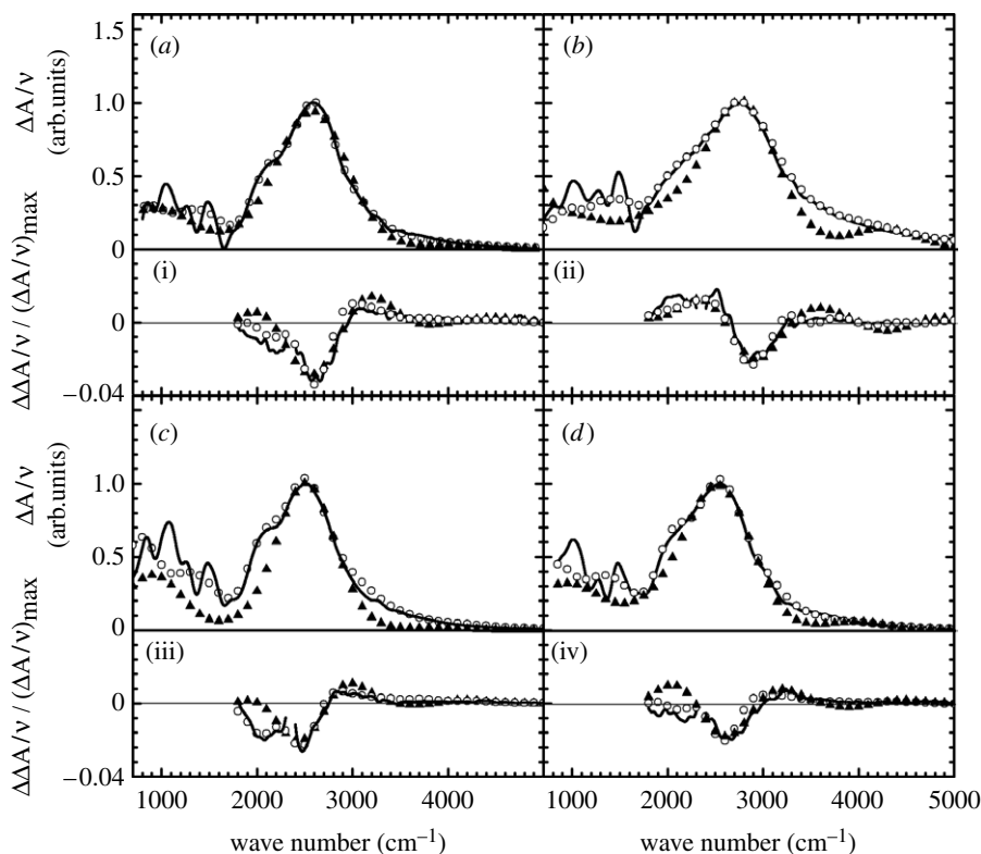
Figure 7. (a–d) Absorption, WT, M160LH, L131LH and M160LH/L131LH, respectively, and (i–iv) Stark spectra of wild-type and mutant RCs as dehydrated protein films at 77 K. Data (lines), fits to the 2-state-1-mode non-classical model (triangles), and fits to the 4-state-70-mode non-classical model (circles) are shown.
