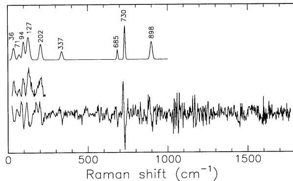
FIG. 4. Rapid-flow resonance Raman spectra of R. sphaeroides (R-26) RCs with 850-nm excitation. At bottom is the complete difference spectrum from 30\text{ cm}^{-1} to 1760\text{ cm}^{-1} . The high-frequency data are shown to demonstrate that no large Raman lines are present above 898\text{ cm}^{-1} . Small Raman features could be masked by the noise above 1000\text{ cm}^{-1} , and no attempt was made to fit the data in this region. The middle spectrum is a flat-field-corrected and background-subtracted spectrum that exposes the 36\text{-cm}^{-1} feature. At top is a simulated spectrum using the Gaussian parameters obtained by fitting reproducible features in the difference spectrum. The approximate relative intensities of the modes that were fit are 0.4, 0.2, 0.6, 1.0, 0.6, 0.3, 0.2, 0.7, and 0.7 for the 36 , 71 , 94 , 127 , 202 , 337 , 685 , 730 , and 898\text{ cm}^{-1} modes, respectively, with estimated uncertainties of \pm 25\% . The 71\text{-cm}^{-1} mode may be an overtone peak of the strong 36\text{-cm}^{-1} mode.
