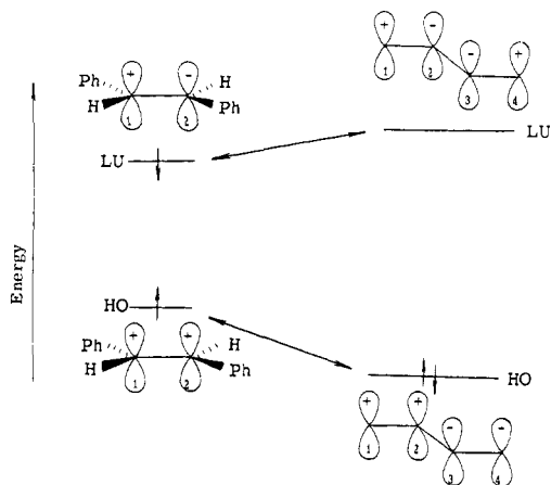
Figure 1. Orbital interaction diagram for excited trans -stilbene with butadiene. Relative energies are estimated from ionization potentials and singlet energies. 17a
