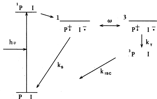
FIG. 1. Simplified scheme for the primary events in quinone-depleted RCs. k_S and k_T are the singlet and triplet radical-pair recombination rate constants; \omega is the singlet-triplet mixing frequency which depends on the magnetic parameters for the radical pair and the field strength. The bar above P^+I^- denotes a spin-correlated radical pair.
